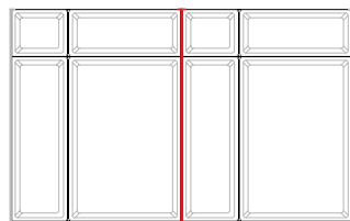
Joint kit for superimposition H180 1ML5210 - 180° 1ML5220 - 90° 1ML5223 - 90° 3-ways 1ML5224 - 90° 4-ways 1ML5230 - 120° 1ML5233 - 120° 3-ways
