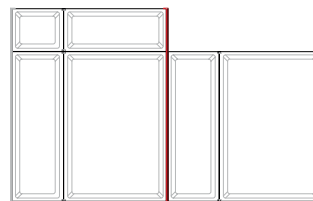
Joint kit for superimposition on right/left H180 1ML5410 - 180° 1ML5320/1ML5420 - 90° right (..420) / left (..320) 1ML5323/1ML5423 - 90° 3-ways right (..423) / left (..323) 1ML5330/1ML5430 - 120° right (..430) / left (..330) 1ML5333 - 120° 3-ways with superimposition on one way 1ML5433 - 120° 3-ways with superimposition on two way
